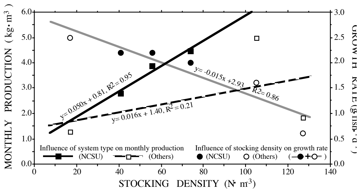
Fig. 3. Comparison of type of integrated recirculatory aquaculture system on fish growth rate and on monthly production per unit volume regressed on stocking density.
