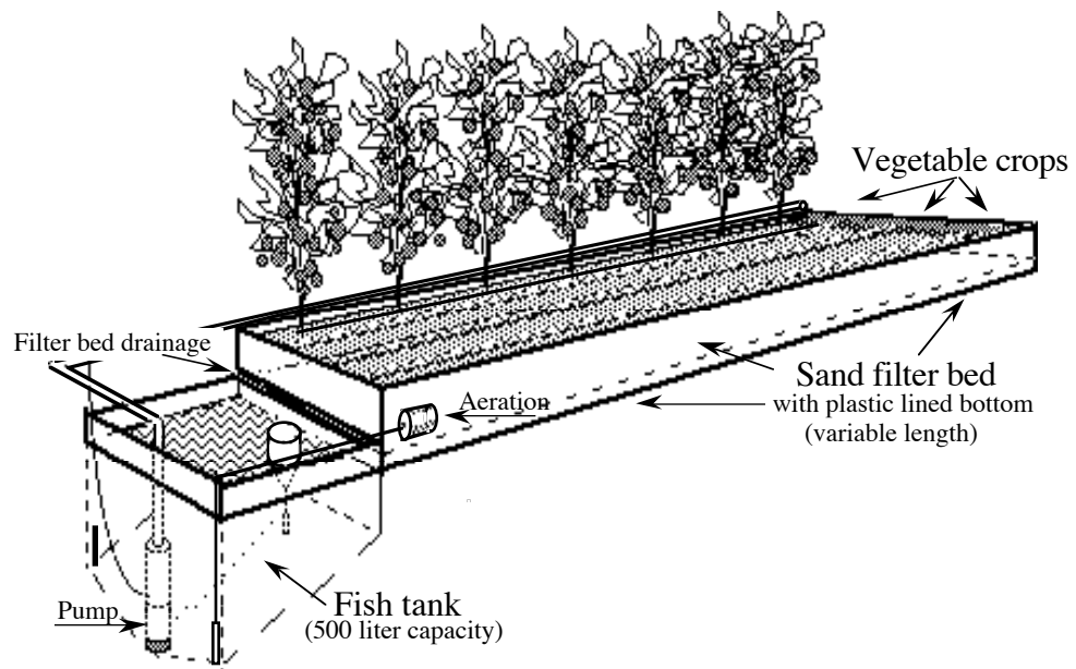
Fig. 1. Schematic diagram of the integrated aquaculture-olericulture system.
